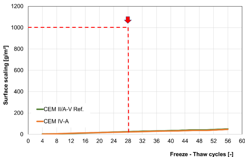
Figure 6: Surface scaling determined using the EN 12390-9 slab test method
