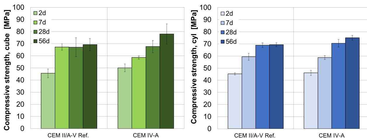
Figure 2. Compressive strength development of CEM II/A-V 52.5 R and CEM IV/A (V) 52.5 R concrete mixes tested in cubes (left) and in cylinders (right) samples.
