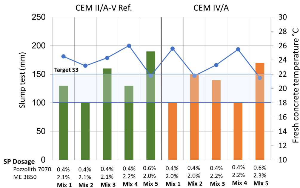
Figure 1. Consistency of CEM II/A-V 52.5 R and CEM IV/A (V) 52.5 R concrete mixes.
