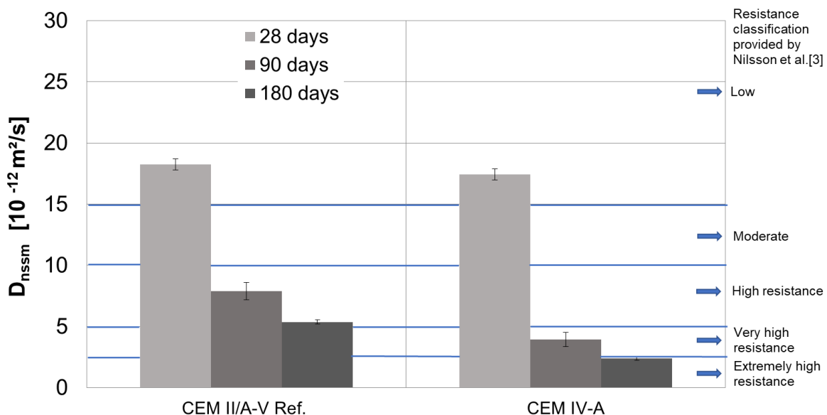
Figure 5: Average chloride migration coefficient measured by RCM test according to NT Build 492, after 28 days, 90 days and 180 days of curing for CEM II/A-V 52.5 R and CEM IV/A (V) 52.5 R concrete mixes.
