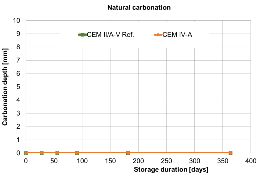
Figure 9: Carbonation depths of CEM II/A-V 52.5 R and CEM IV/A (V) 52.5 R concrete mixes. Natural carbonation: exposed to laboratory conditions 20 °C / 65% RH for 365 days.
