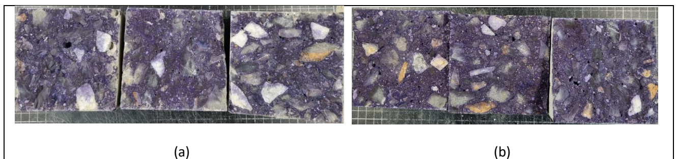
Figure A. 10: Accelerated carbonation of (a) three CEM II/A-V (Ref.) and (b) three CEM IV/A(V) samples after 28 days of testing
