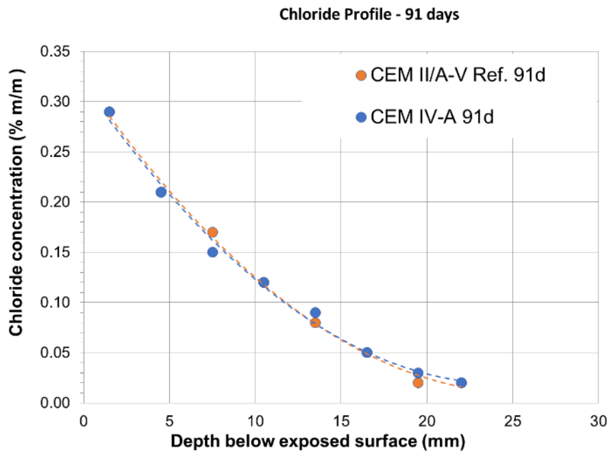
Figure 4. Chloride profile of CEM II/A-V 52.5 R and CEM IV/A (V) 52.5 R concrete mixes according to EN 12390-11, exposed for 91 days in 3% NaCl solution.
