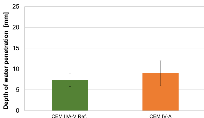
Figure 10: Water penetration depths of CEM II/A-V 52.5 R and CEM IV/A (V) 52.5 R concrete mixes.
