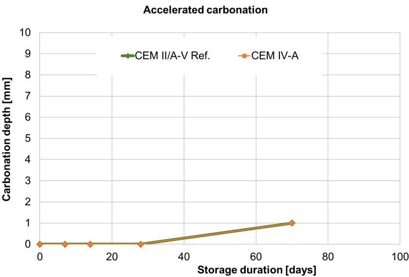
Figure 8: Accelerated carbonation of CEM II/A-V 52.5 R and CEM IV/A (V) 52.5 R concrete mixes.
