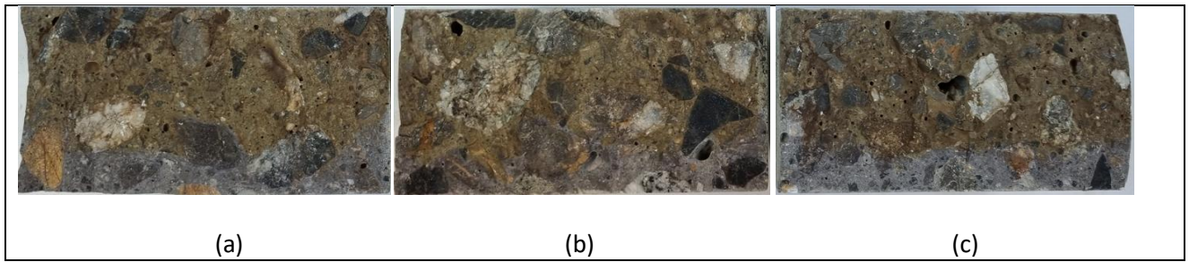
Figure A. 3: Chloride migration front of CEM II/A-V (Ref.) individual samples after 180 days of curing
